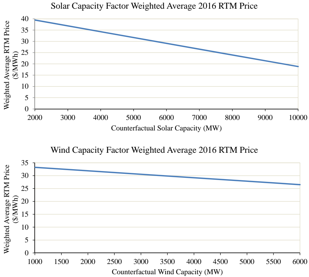
Figure 9: The top panel displays the weighted average of the predicted 2016 hourly RTM prices for different levels of installed solar capacity. Each hourly predicted price is weighted by the share of 2016 solar generation that would occur during the specific hour. Similarly, the bottom panel displays the weighted average of the predicted 2016 RTM prices for different levels of wind capacity. Again, the weights are the share of total annual wind generation that occurs during the specific hour.
